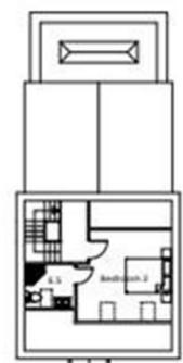
Second Floor Plan No. 1
