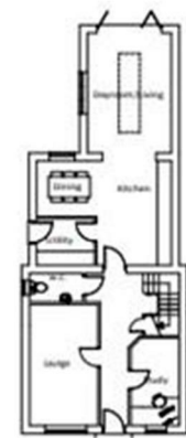
Ground Floor Plan No. 2
